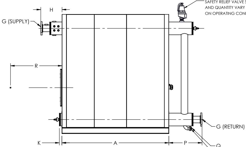
SIDE VIEW
