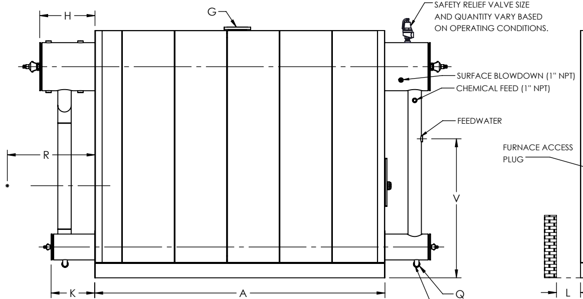
SIDE VIEW
